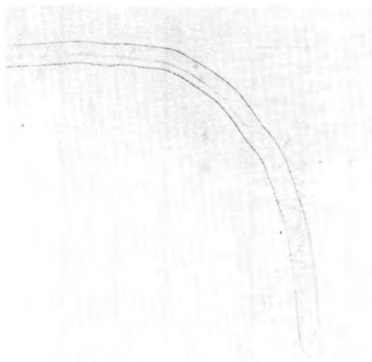
Fig. 4. The gravitropic arc
