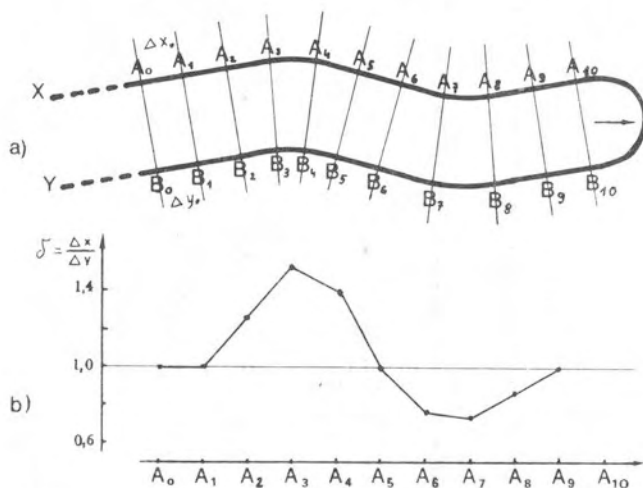
Fig. 1. Scheme of the assignment of curvature changes along the rhizoid
