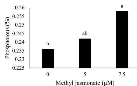
Fig. 1 Effect of methyl jasmonate on phosphorus percentage in tomato leaves.
