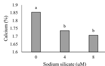
Fig. 2 Effect of sodium silicate on calcium percentage in tomato leaves.
